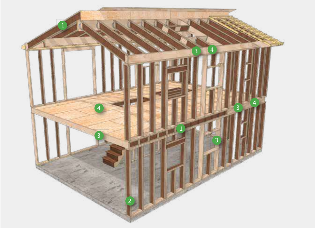
STEICO I-joists
